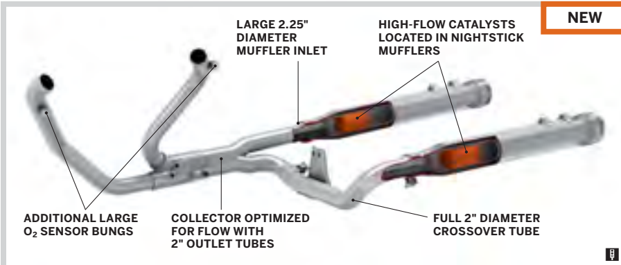
C. SCREAMIN' EAGLE HIGH-FLOW EXHAUST SYSTEM WITH NIGHTSTICK MUFFLERS
