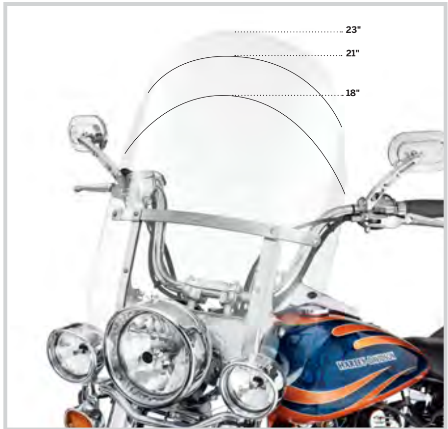
A. KING-SIZE H-D DETACHABLES WINDSHIELD FOR FL SOFTAIL MODELS WITH AUXILIARY LIGHTING – POLISHED BRACES
