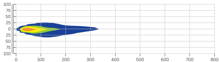
Original Equipment Halogen Low Beam (7") Birds Eye View (shown in feet)
