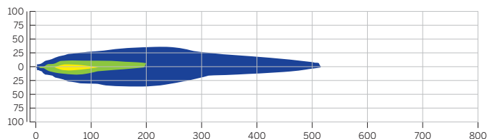
Original Equipment Halogen High Beam (7") Birds Eye View (shown in feet)
