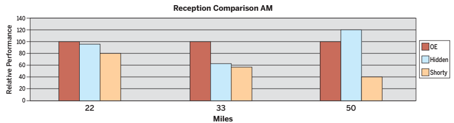
ANTENNA PERFORMANCE COMPARISON – COMPARISON MEASURED ON '06-'13 MODELS WITH ADVANCED AUDIO AM/FM/WB RADIO
